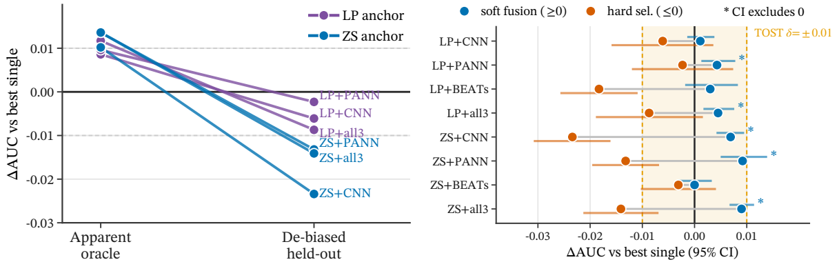
Figure 4: Headroom-audit detail. Left: selection-overfit anatomy, tracing six cells (BEATs omitted for readability) from apparent oracle \Delta AUC to de-biased held-out \Delta AUC ; the held-out estimates collapse below zero. Purple denotes the LP anchor and blue denotes the ZS anchor. Right: calibrated soft-fusion \Delta AUC (blue, * CI excludes 0 in 5/8 cells) compared with de-biased hard-selection \Delta AUC (red).
