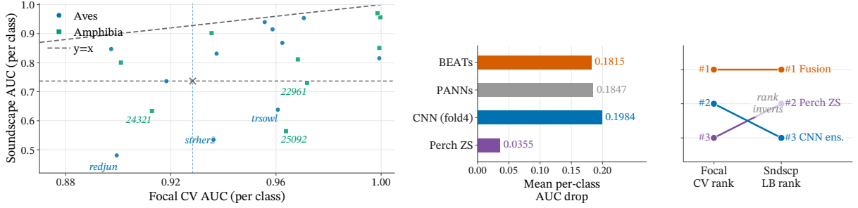
Figure 5: Domain-shift diagnostics. Left: focal-CV AUC versus soundscape AUC for the 20 most-affected of 47 common scorable classes under Perch V2 zero-shot (circle=Aves, square=Amphibia); redjun drops 0.899 \rightarrow 0.481, the 47-class shared mask drops from 0.928 to 0.889, the 75-class soundscape macro-AUC is 0.737, and \text{RBF-MMD}^2=0.092 . Right: robustness gap and CV-LB rank inversion. Perch ZS has the smallest mean per-class focal \rightarrow soundscape AUC drop on the matched 43-class fold-4 mask (0.0355 versus CNN 0.198, PANNs 0.185, BEATs 0.182), and Perch ZS and the CNN ensemble swap rank between focal CV and the soundscape LB validation track ( n=3 , qualitative).
