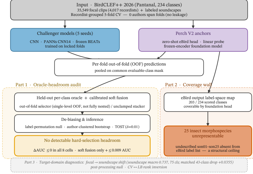
Figure 1: Three-part audit pipeline. Recordist-grouped 5-fold splits feed two Perch V2 anchors (zero-shot, linear probe) and three trained challengers (CNN, PANNs, BEATs), producing out-of-fold predictions on a common evaluable mask. Part 1 (oracle-headroom audit): a held-out per-class oracle and calibrated soft fusion, de-biased by a label-permutation null and author-clustered bootstrap with TOST tests, yield no detectable hard-selection headroom across the 8 cells. Part 2 (coverage wall): the Perch V2 eBird output head cannot represent 25 undescribed insect morphospecies, a structural ceiling. Part 3 (target-domain diagnostics): focal-to-soundscape tests check whether focal-CV conclusions transfer to soundscapes. Quantities appear in the corresponding Results subsections.
